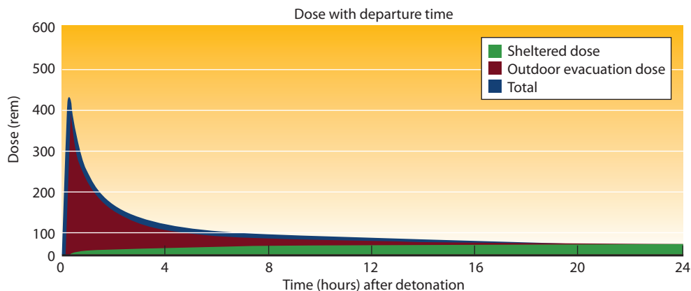
Figure 32. Exposures in good-quality shelter near St. Vincent's Medical Center.
